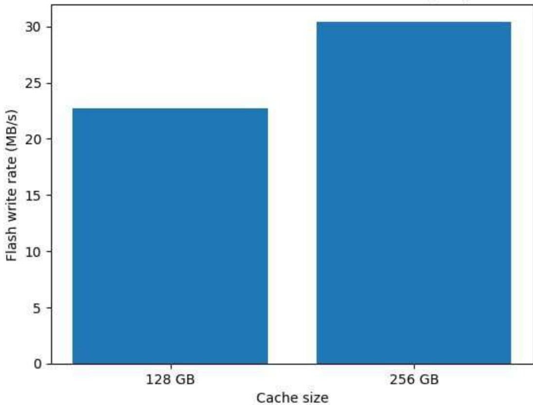
Effect of cache size on flash write rate (LRU)
